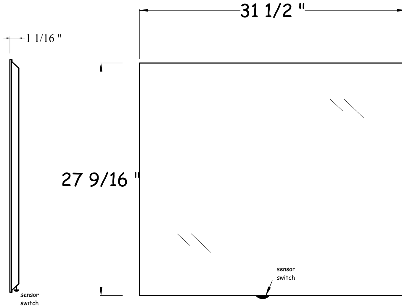
Front View
