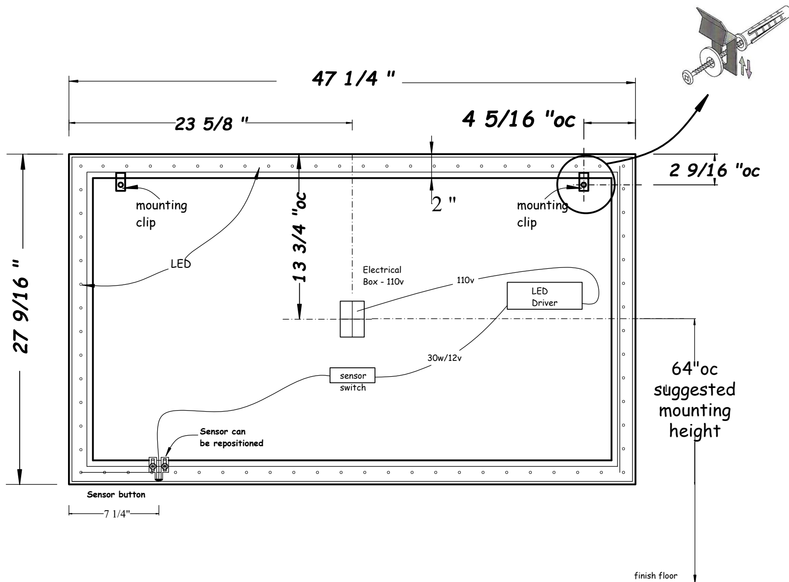
Rear View
