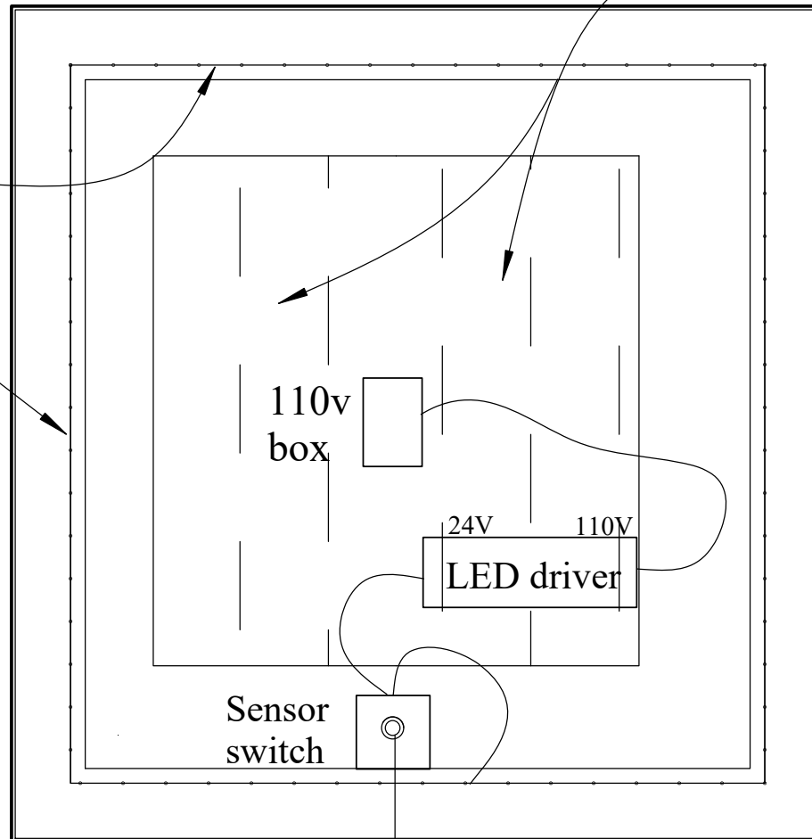
Rear View
