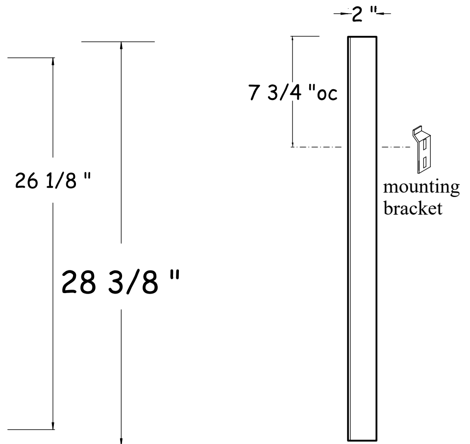
Section View
