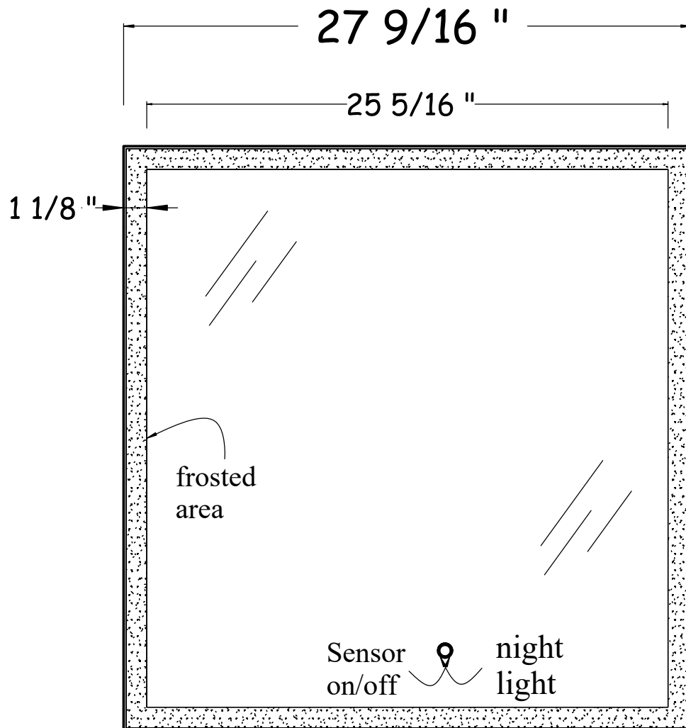
Front View
