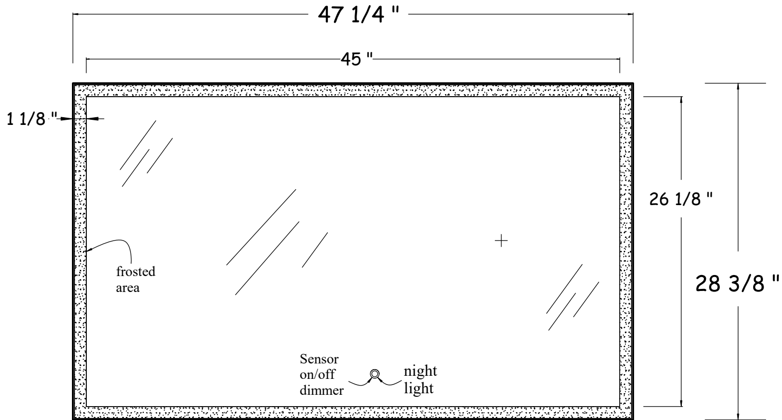
Front View
